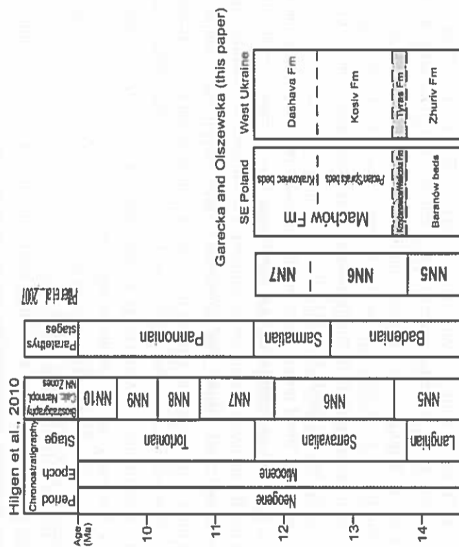
Fig. 1. Biostratigraphical scheme of the investigated Miocene deposits of the SE part of the Polish and NW part of the Ukrainian Carpathian Foredeep (Bilche-Volytsia Zone).
